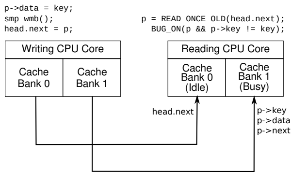
Figure 15.15: Why smp_read_barrier_depends() is Required in Pre-v4.15 Linux Kernels
