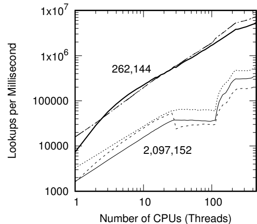
Figure 10.19: Overhead of Resizing Hash Tables Between 262,144 and 524,288 Buckets vs. Total Number of Elements
