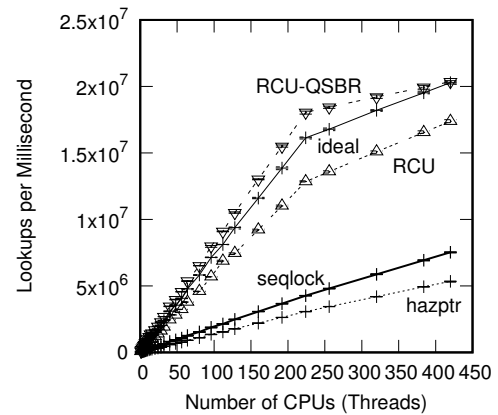
Figure 9.22: Pre-BSD Routing Table Protected by RCU QSBR
