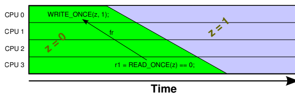
Figure 15.10: Load-to-Store is Counter-Temporal
