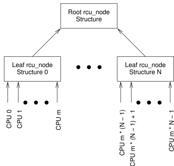
Figure 7.8: Locking Hierarchy
