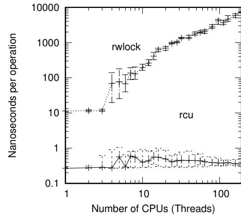
Figure 9.23: Performance Advantage of RCU Over Reader-Writer Locking
