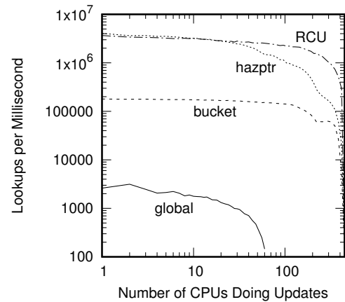
Figure 10.11: Read-Side RCU-Protected Hash-Table Performance For Schrödinger's Zoo in the Presence of Updates
