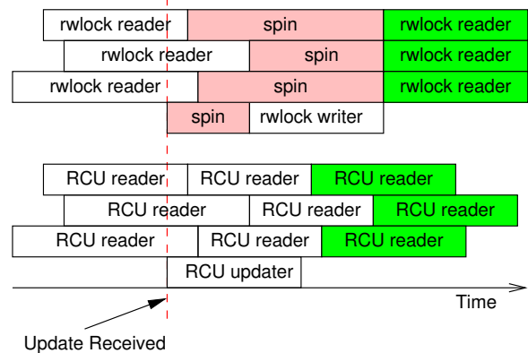
Figure 9.26: Response Time of RCU vs. Reader-Writer Locking
