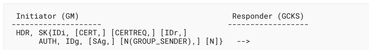
Figure 3: GSA_AUTH Request
