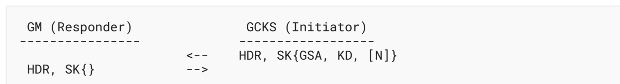
Figure 11: GSA_INBAND_REKEY Exchange
